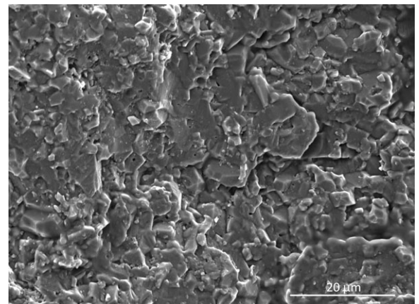
Fig. 8. A representative tensile fracture surface for a sintered 55 vol.% alumina suspension. Mostly transgranular fracture is observed, with no delamination between deposited filament layers.
