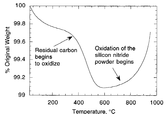
Fig. 3. Thermogravimetric response of a ceramic powder/residual carbon sample heated in flowing air from room temperature through 900°C. Sharp decrease in weight beginning near 400°C is due to oxidation of residual carbon.
