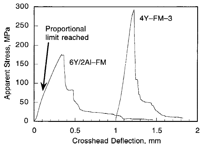
Fig. 8. Flexural response comparison of a 4Y-FM-3 and 6Y/2Al-FM tested at 1400°C. Proportional limit was reached at only 65 MPa for the 6Y/2Al-FM.
